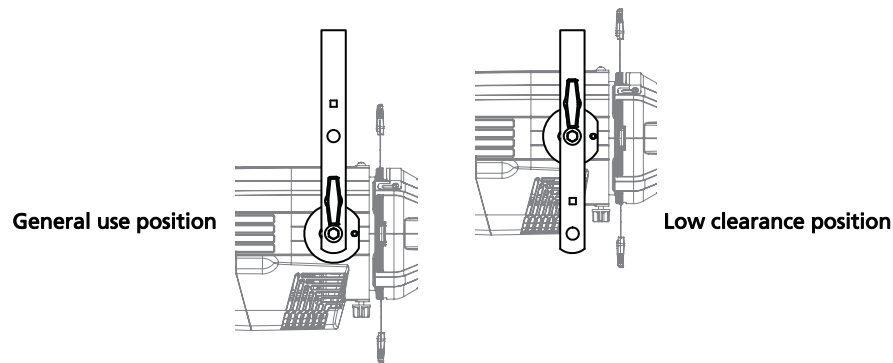
Figure-2.10 Adjusting the yoke position
