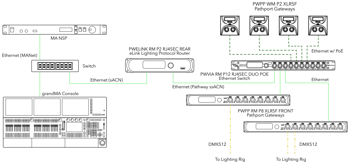
Example of a network using the Guest On-Ramp application. Note the MANet data never reaches the downstream system.
