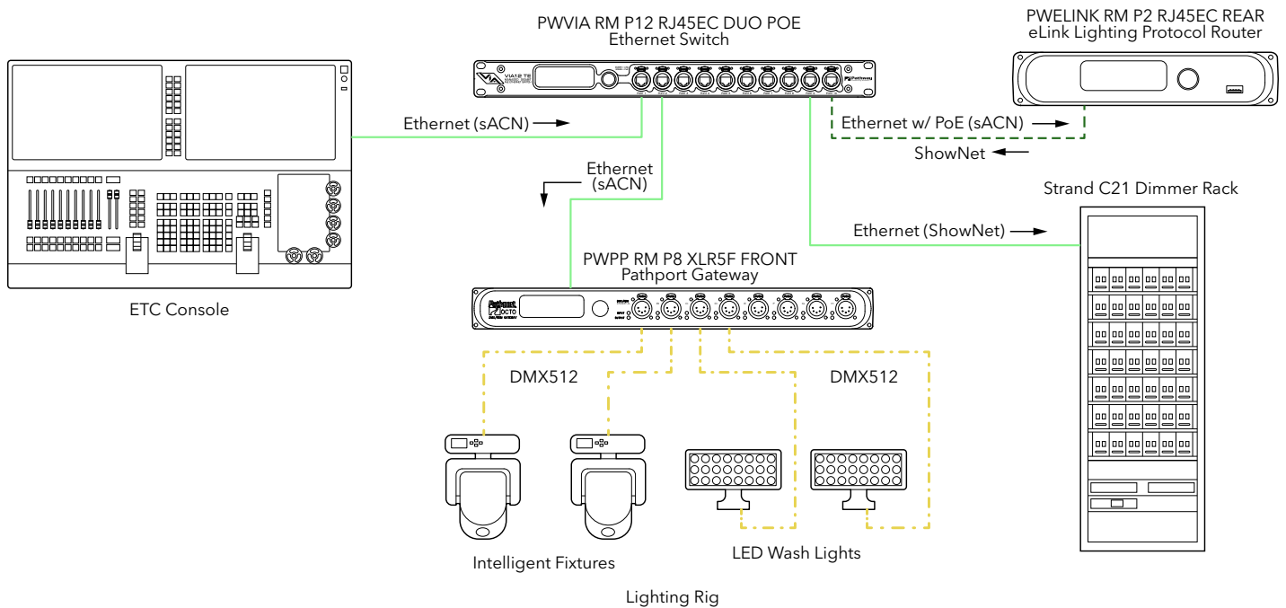
Example of a network transmitting converted protocols back onto the primary NIC for integrating a C21 dimmer rack into an sACN system
