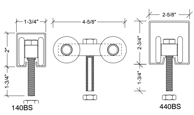
No. 140BS & 440BS Scenery Carrier
