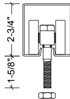
No. 450 Urethane Scenery Carrier
