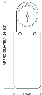
No. 643 Sand Bag Tension Pulley
