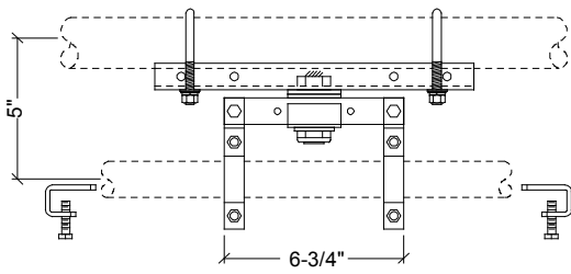
No. 6 Pivot Device
