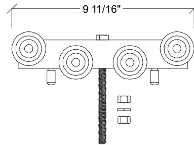
No. 450A Urethane Scenery Carrier
