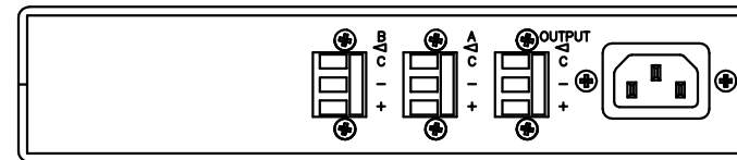
model 221E-TB REAR TWO PART SEPARATING TERMINAL BLOCK
