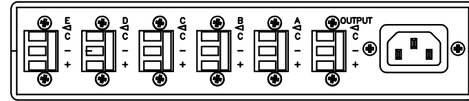
model 521E-TB REAR TWO PART SEPARATING TERMINAL BLOCK
